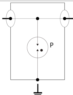
P: 2-electrode gas discharge tube
