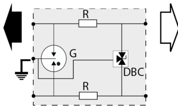
Gb: 3-electrode gas tube R: Resistor DBC: 3-pole low capacitance diode
