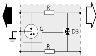
G: 3-electrode gas tube R: Resistor D3: 3-pole clamping diode
