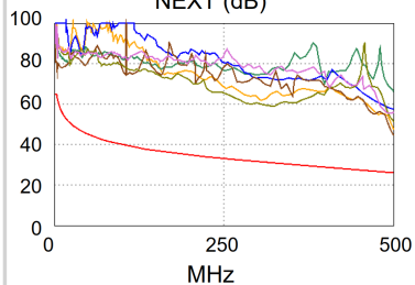
G: 3-electrode GDT NEXT (dB)
