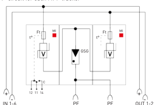
"MOV" circuit for each MPP tracker
